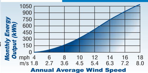
Rayleigh Distribution Curve k=2
