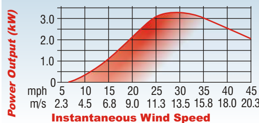
Performance Curves
